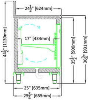
A - 25 3/4" D (655mm) SIDE VIEW
