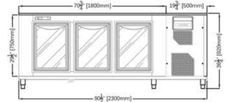
UCW2300
