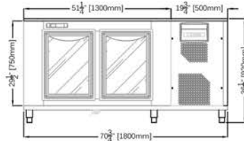
UCW1800
