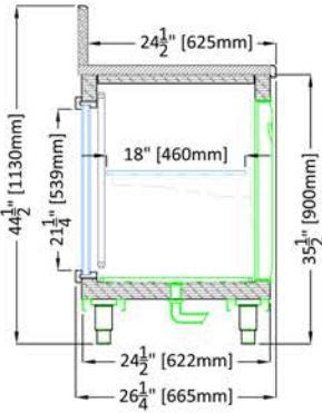
A - 26 1/4" D (665mm) SIDE VIEW
