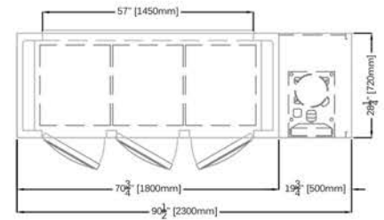
UCW2300
