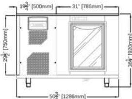
UCW1300
