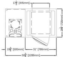
UCW1300
