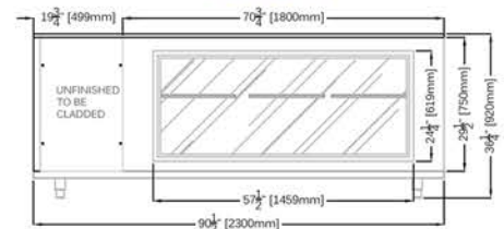
UCW2300
