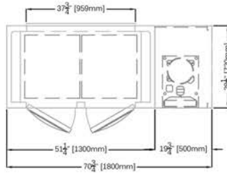
UCW1800
