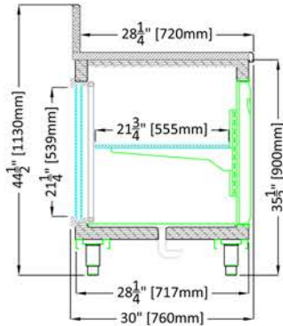
B - 30" D (760mm) SIDE VIEW
