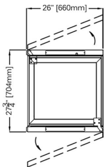
VC6314D H60/H76
