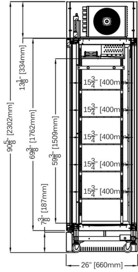
SECTION VIEW
