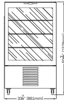
VN8314 H60
