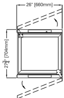
V6314D H60/H76
