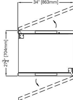
VN8314D H60/H76
