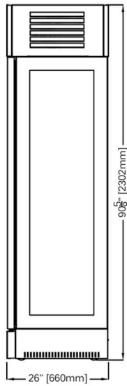
RIGHT SIDE
