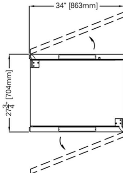
VC8314D H60/H76
