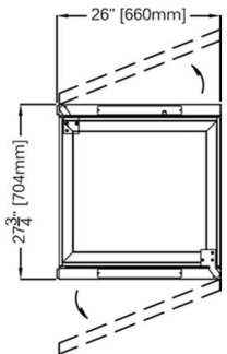
VN6314D H60/H76
