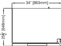
VN8314 H60/H76
