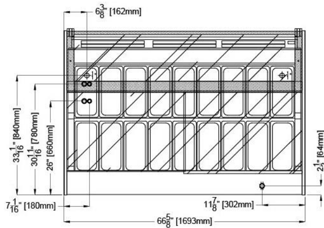
DIAMOND PRO 1-2-3 G1650
