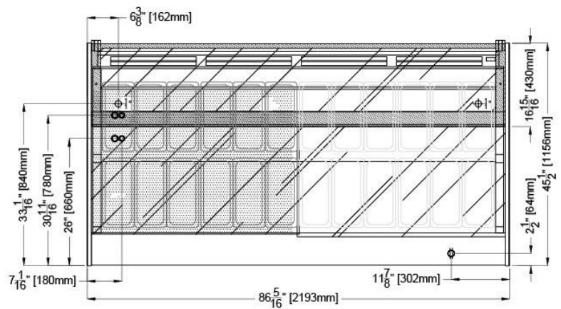
DIAMOND PRO 1-2-3 G2150 Dual Temp
