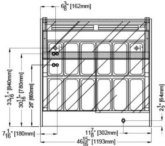
DIAMOND PRO 1-2-3 G1150
