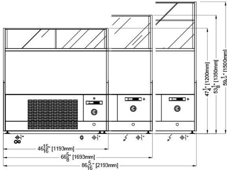
DIAMOND PRO 1-2-3 G2150 Dual Temp
