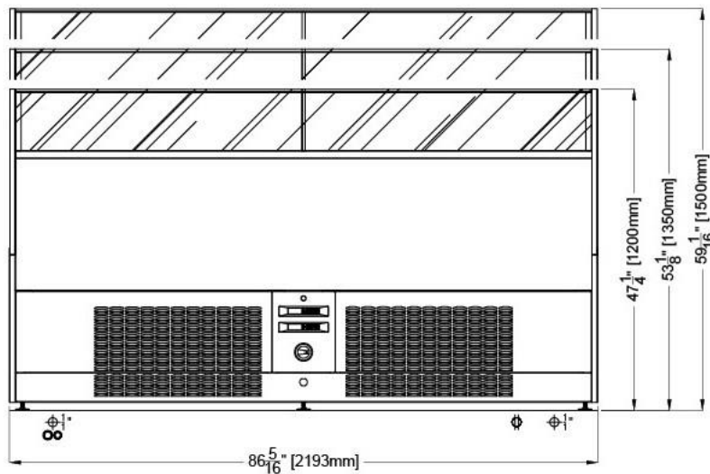
DIAMOND PRO 1-2-3 G2150 Dual Temp
