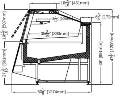
METRO 1 - 47 1/4"H
