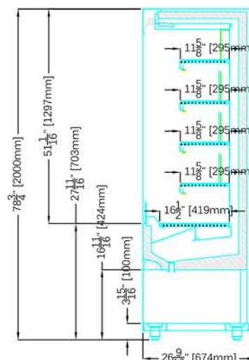
SQ TYPE
